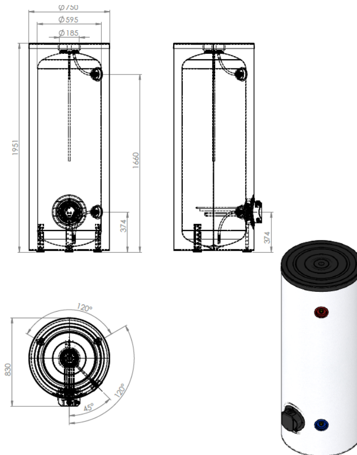
Figure 1 – Dimensions
