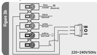
Wiring connection diagram for models with flange diameter 315 (for fans with speed switch button)
