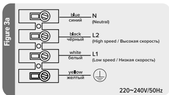
Wiring connection diagram for models with flange diameter 315 (for fans without speed switch button)
